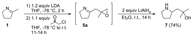
Scheme 3.
